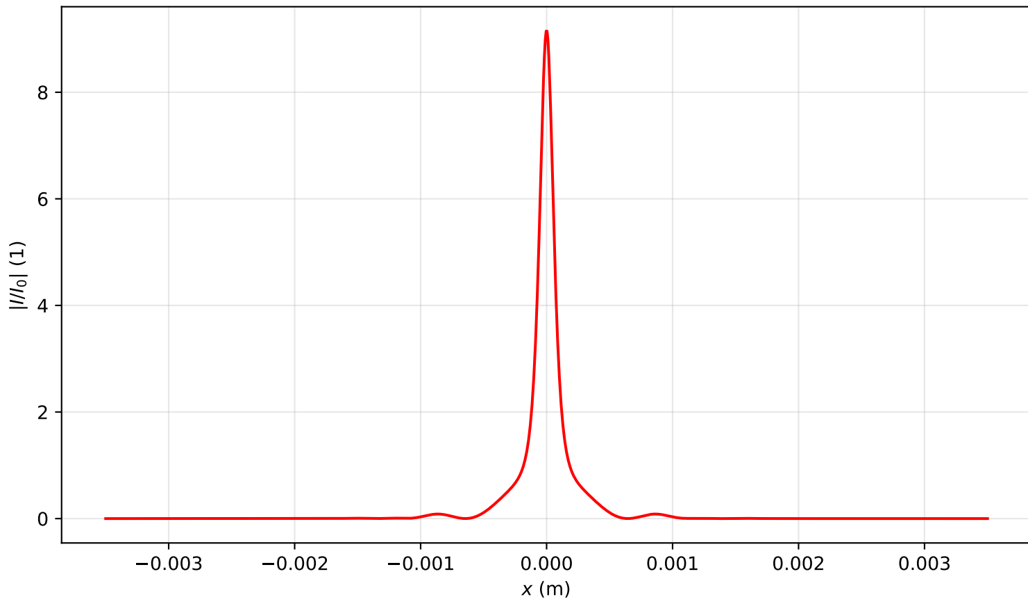
Intensity profile I(x, y = 0, z = 1.194)/I_0 , P_{in}=4.0P_{cr} , artificial time
